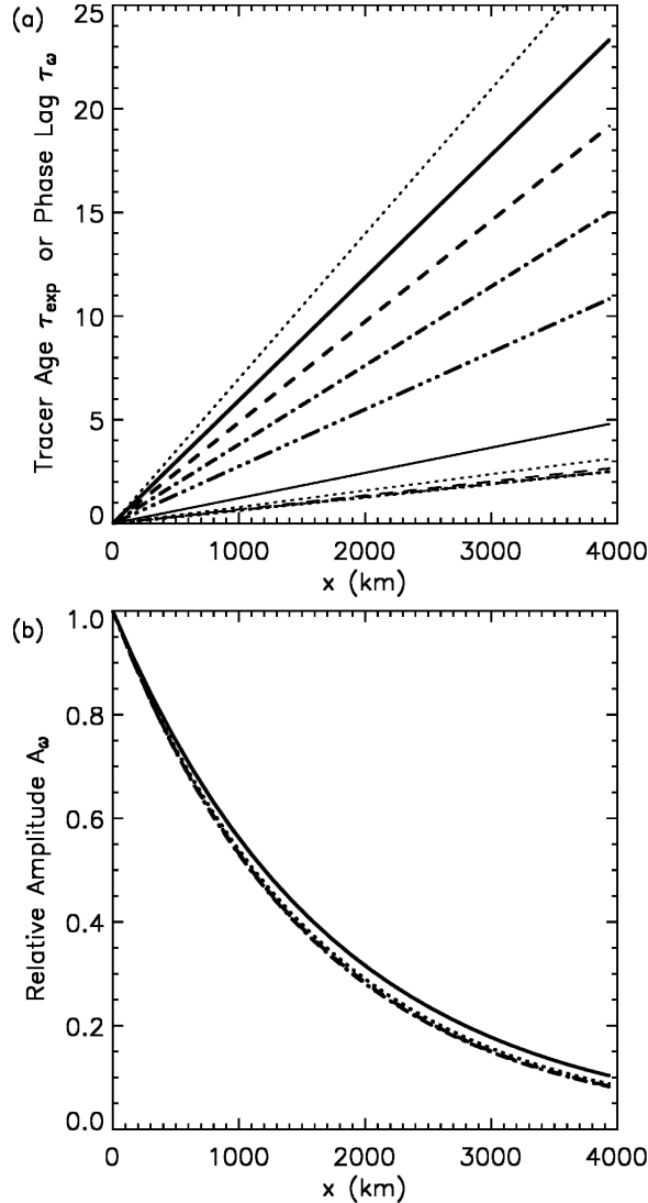
FIG. 5. Variation of (a) mean transit time \Gamma , age of exponential tracer \tau_{exp} , and phase lag of periodic tracer \tau_{\omega} and (b) amplitude of period tracer A_{\omega} with x for \alpha = 0.1 , u = 5 \text{ cm s}^{-1} , and mixing time t_{mix} = 1.0 \text{ yr} . The upper set of curves in (a) show \Gamma (dotted curve) and tracer age with T_{exp} = 50 (solid curve), 20 (dashed), 10 (dot-dashed), and 5 (triple dot-dashed) yr, whereas the lower set of curves show the phase lag for T_{\omega} = 20 (solid), 10 (dotted), 5 (dashed), and 1 (dot-dashed) yr.
