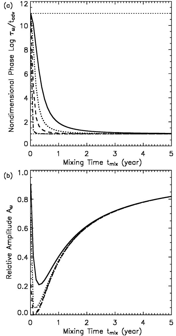
FIG. 6. Variation of (a) phase lag \tau_{\omega} and (b) amplitude A_{\omega} of periodic tracers with mixing time t_{mix} for periods equal to 20 (solid), 10 (dotted), 5 (dashed), and 1 (dot-dashed) yr. In both plots \alpha = 0.1 and t_{adv} = 1 \text{ yr} .
