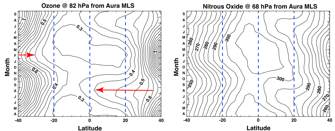
Figure 8. Latitude/time plot of mixing ratio of (a) 82 hPa ozone and (b) 68 hPa N_2O from the measurements on Aura MLS. Ozone mixing ratios are in parts per million by volume, and nitrous oxide mixing ratios are in parts per billion by volume. Results are from a monthly mean climatology in 2^\circ latitude bands repeated with 18 months shown from April through September. Red arrows are drawn from the 0.6 contour to the 0.4 contour in the summer of the northern and southern tropics to emphasize the apparent strong mixing into the northern tropics. Blue dashed lines are drawn at 20^\circ S , equator, and 20^\circ N to show the two tropical regions considered in the analysis.
