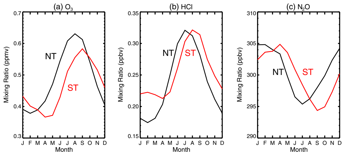
Figure 5. Mean seasonal cycle for (a) O_3 , (b) HCl, and (c) N_2O at 68 hPa in the NT and ST as measured by Aura MLS.
