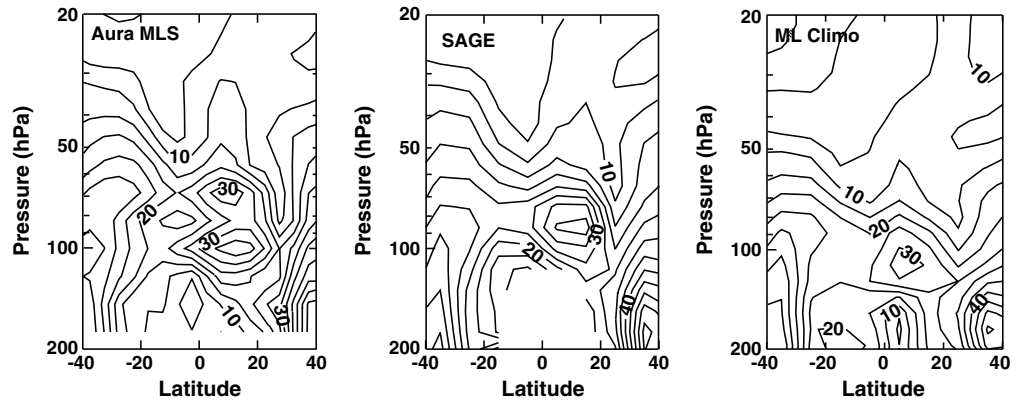
Figure 4. Latitude-altitude dependence of the magnitude of the annual cycle in ozone, in percent of the mean value, for (a) 8 years of Aura MLS data, (b) 21 years of SAGE II data, and (c) McPeters and Labow [2012] climatology.
