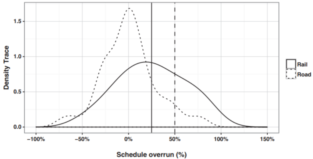
Figure 6. Density trace of schedule overruns by project type and mean (vertical lines) – road (n=74) and rail (n=21)
