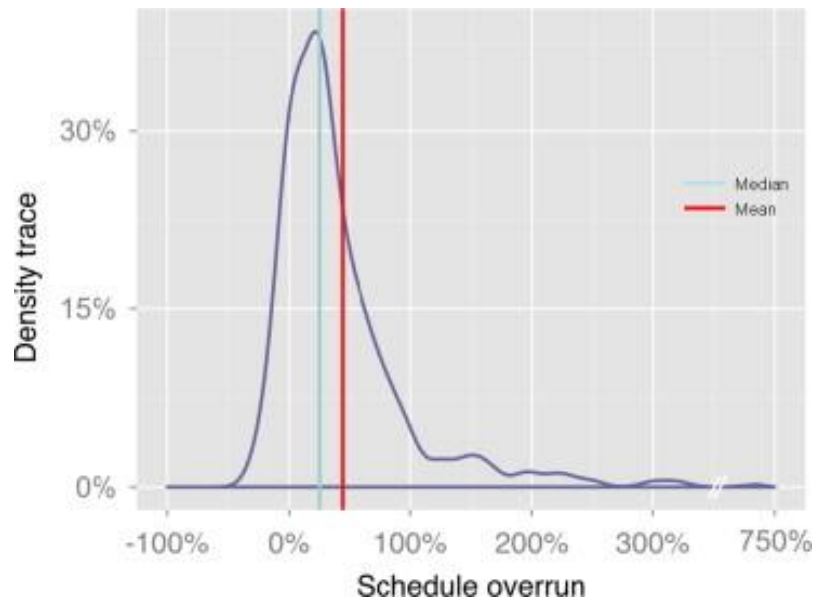
Figure 11. Inaccuracy of schedule estimates (local currencies, constant prices) for large dams over time (N=245), 1934–2007.
