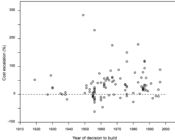
Figure 3. Inaccuracy of cost estimates in transportation projects over time, 1910-1998 (fixed prices, 111 projects)
