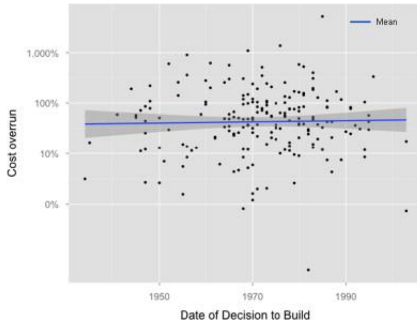
Figure 10. Inaccuracy of cost estimates (local currencies, constant prices) for large dams over time (N=245), 1934–2007.
