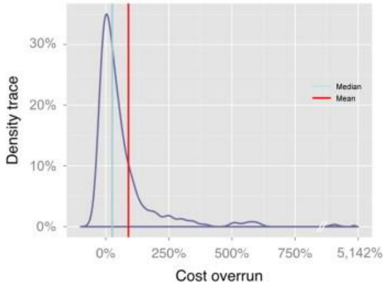
Figure 8. Density trace of actual/estimated cost (i.e. costs overruns) in constant local currency terms with the median and mean (N=245).
