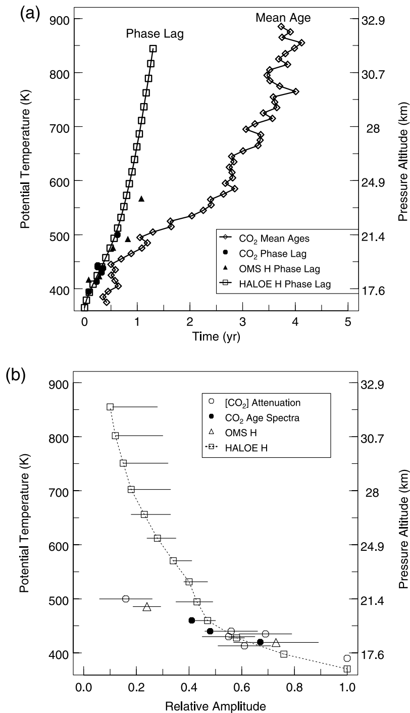
Figure 9. (a) Observational estimates of the vertical variation in the tropical stratosphere of \tau_w for an annual cycle. Squares correspond to \tau_w determined from 4 years of measurements of H 2 O and CH 4 from the Halogen Occultation Experiment (HALOE) [Mote et al. , 1998], the solid triangles correspond to \tau_w from in situ measurements of H 2 O and CH 4 (H. Vomel, personal communication, 2000), and the solid circles correspond to \tau_w from in situ measurements of CO 2 from the ER-2 aircraft [Andrews et al. , 1999]. Also shown are estimates of \Gamma from balloon measurements of CO 2 . (b) Observed amplitude as a fraction of the tropopause value from HALOE measurements of \hat{H} and from in situ aircraft and balloon measurements of CO 2 and \hat{H} models. (Adapted from Park et al. [1999].)
