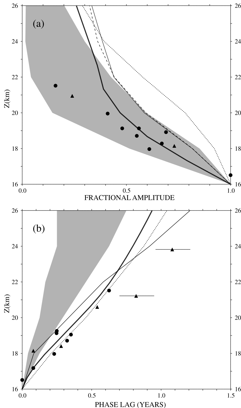
Figure 11. Equatorial profiles of (a) A_\omega(z) and (b) \tau_\omega(z) for a range of models and observations. All amplitudes are normalized to unity, and the phase lag is taken as zero at 16 km. The shaded region indicates the range of most models in the MM2 study, while the individual (thin) lines represent several models falling outside the range. The bold solid line represents the analysis of HALOE \dot{H} [Mote et al. , 1998], and the symbols represent analysis of in situ measurements of \text{CO}_2 (circles) and \dot{H} (triangles). The error bars on the top two in situ phase lag points are estimated from the uncertainty in the tropopause \dot{H} time series. (From Hall et al. [1999].)
