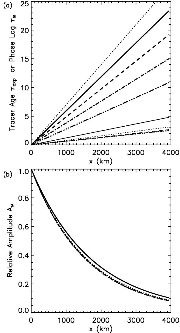
FIG. 5. Variation of (a) mean transit time \tau_{\text{exp}} , age of exponential tracer \tau_{\text{exp}} , and phase lag of periodic tracer \tau_{\omega} and (b) amplitude of periodic tracer A_{\omega} with x for \alpha = 0.1 , u = 5 \text{ cm s}^{-1} , and mixing time t_{\text{mix}} = 1.0 \text{ yr} . The upper set of curves in (a) show \tau_{\text{exp}} (dotted curve) and tracer age with T_{\text{exp}} = 50 (solid curve), 20 (dashed), 10 (dot-dashed), and 5 (triple dot-dashed) yr, whereas the lower set of curves show the phase lag for T_{\omega} = 20 (solid), 10 (dotted), 5 (dashed), and 1 (dot-dashed) yr.
